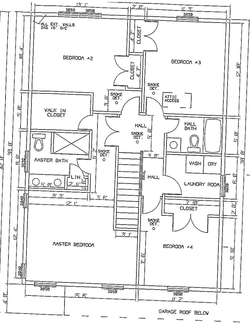
SECOND FLOOR PLAN SCALE: 3/16" = 1"
