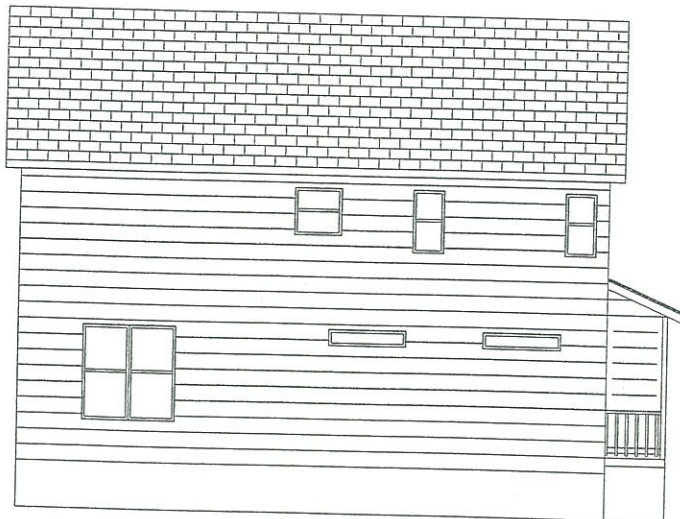
LEFT VIEW
