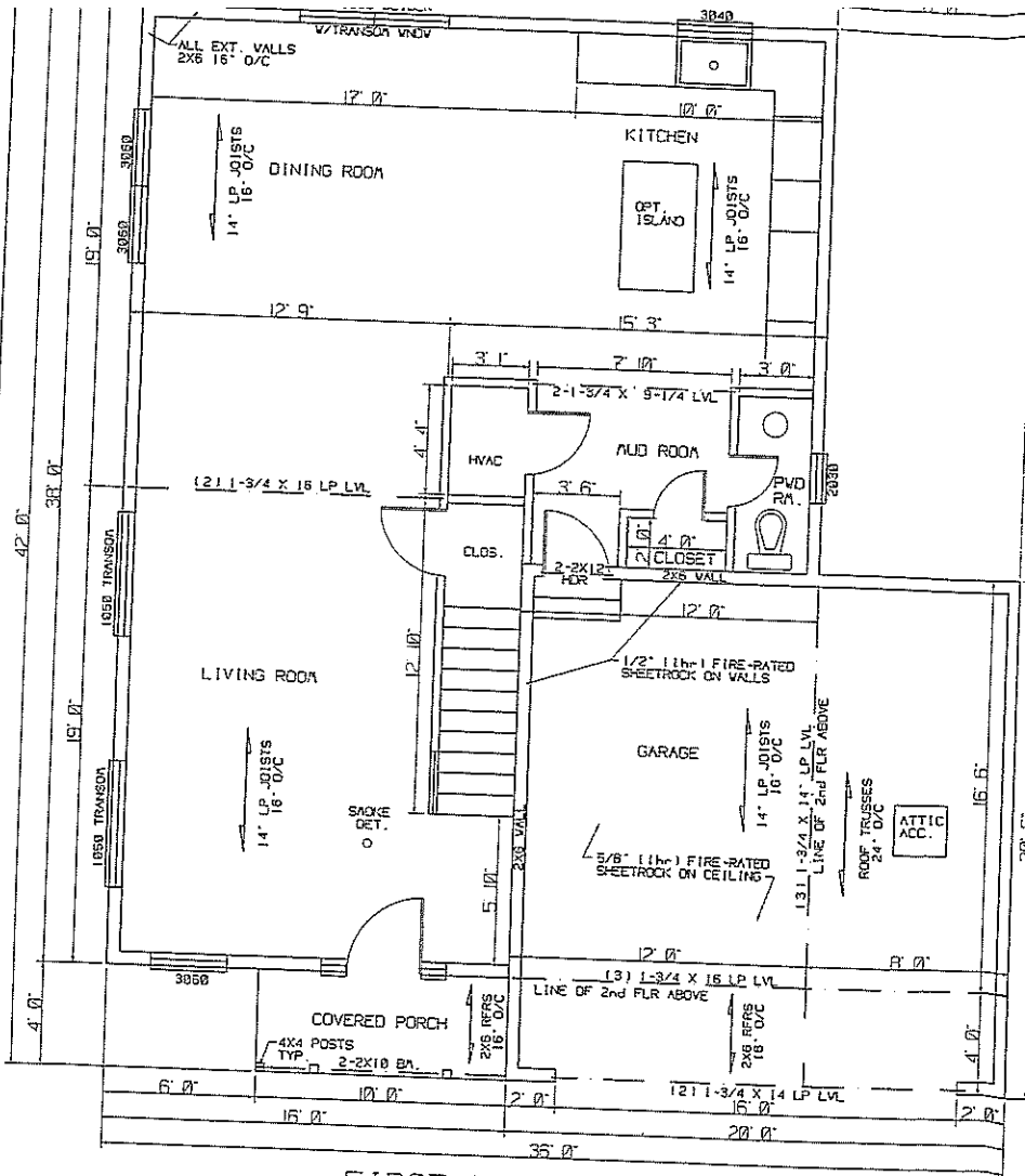
FIRST FLOOR PLAN SCALE: 3/16" = 1"
