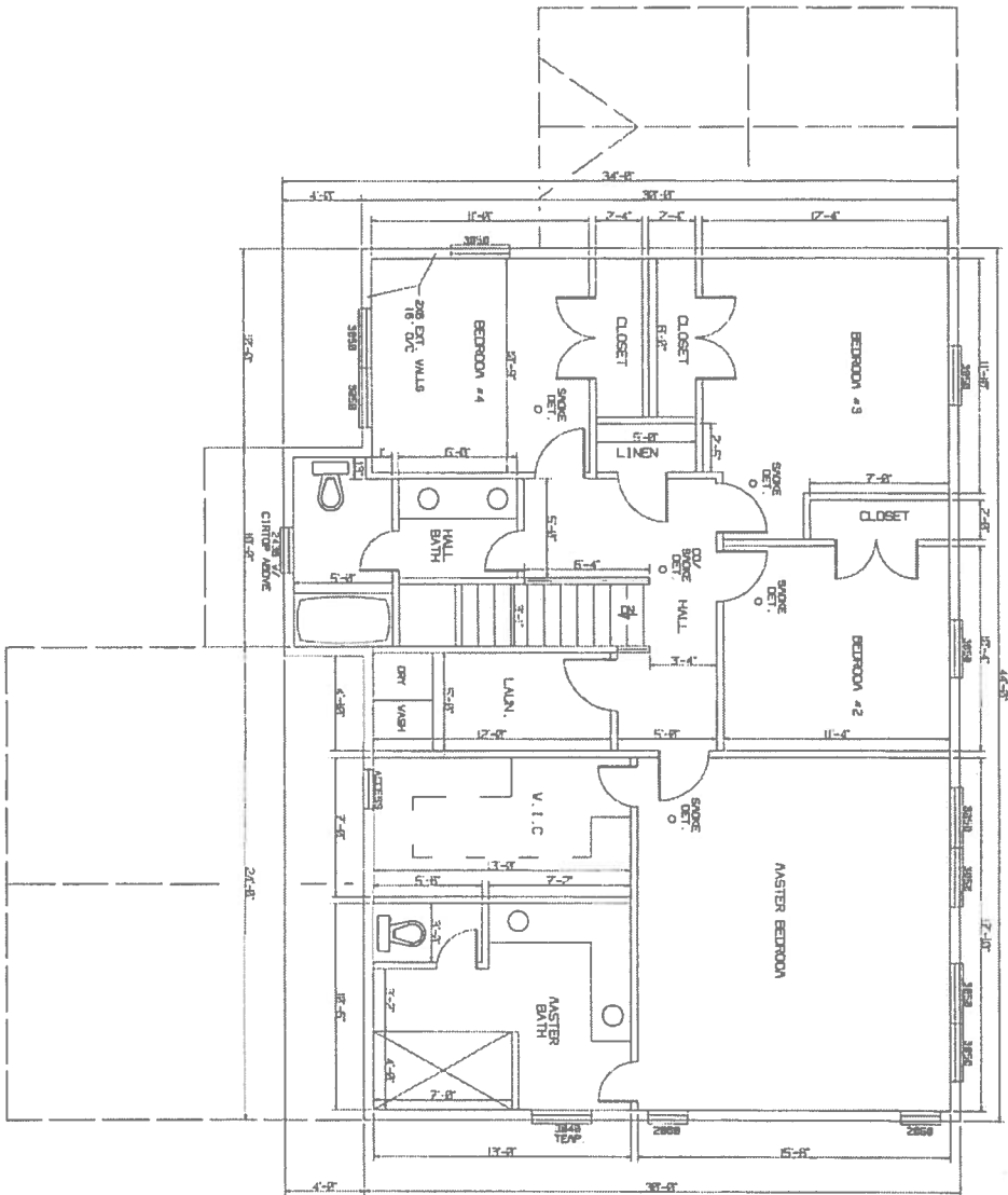
SECOND FLOOR PLAN SCALE: 3/16" = 1'
