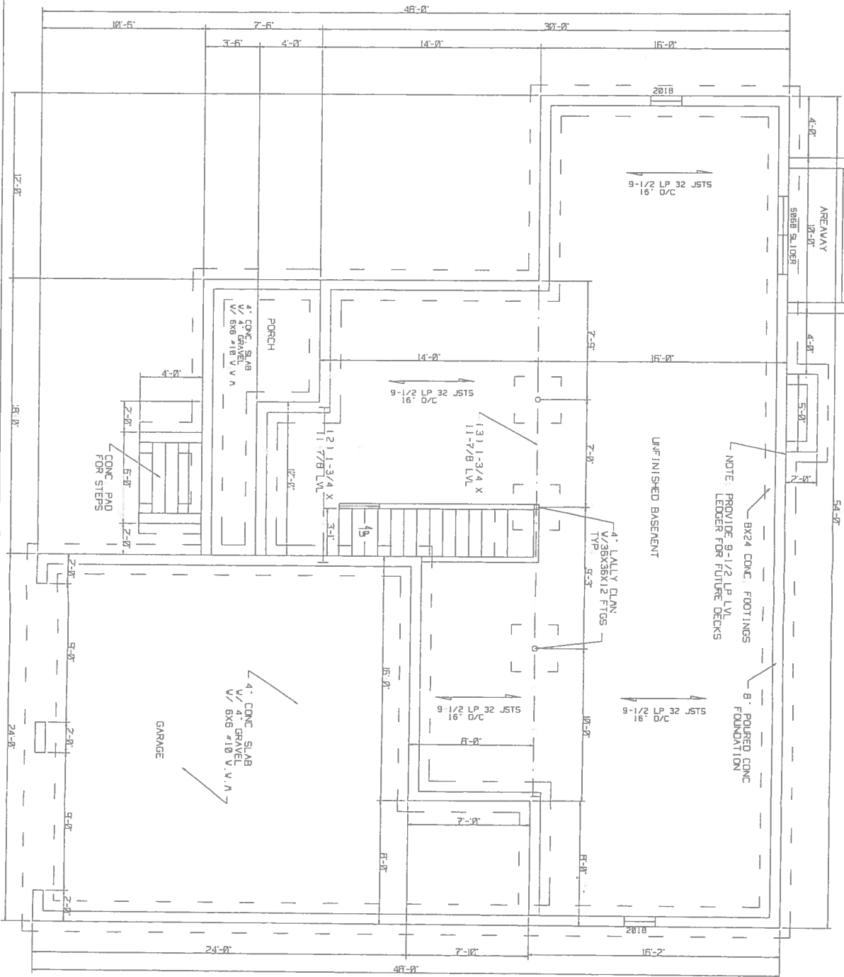
FOUNDATION PLAN SCALE: 3/16" = 1'
