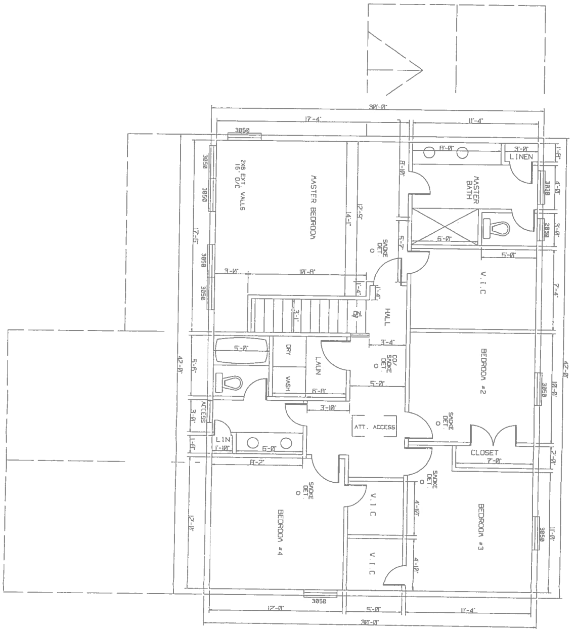
SECOND FLOOR PLAN SCALE 3/16" = 1'
