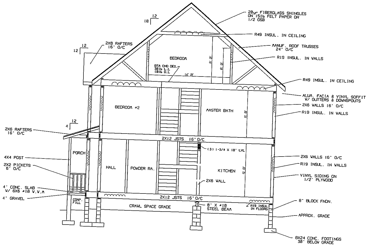
SECTION VIEW SCALE: 3/16" = 1"
