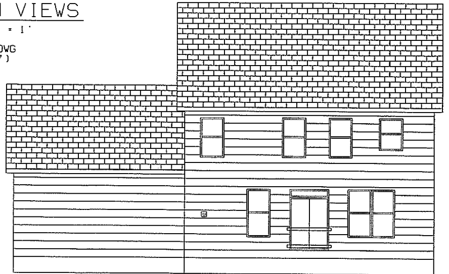
REAR VIEW
