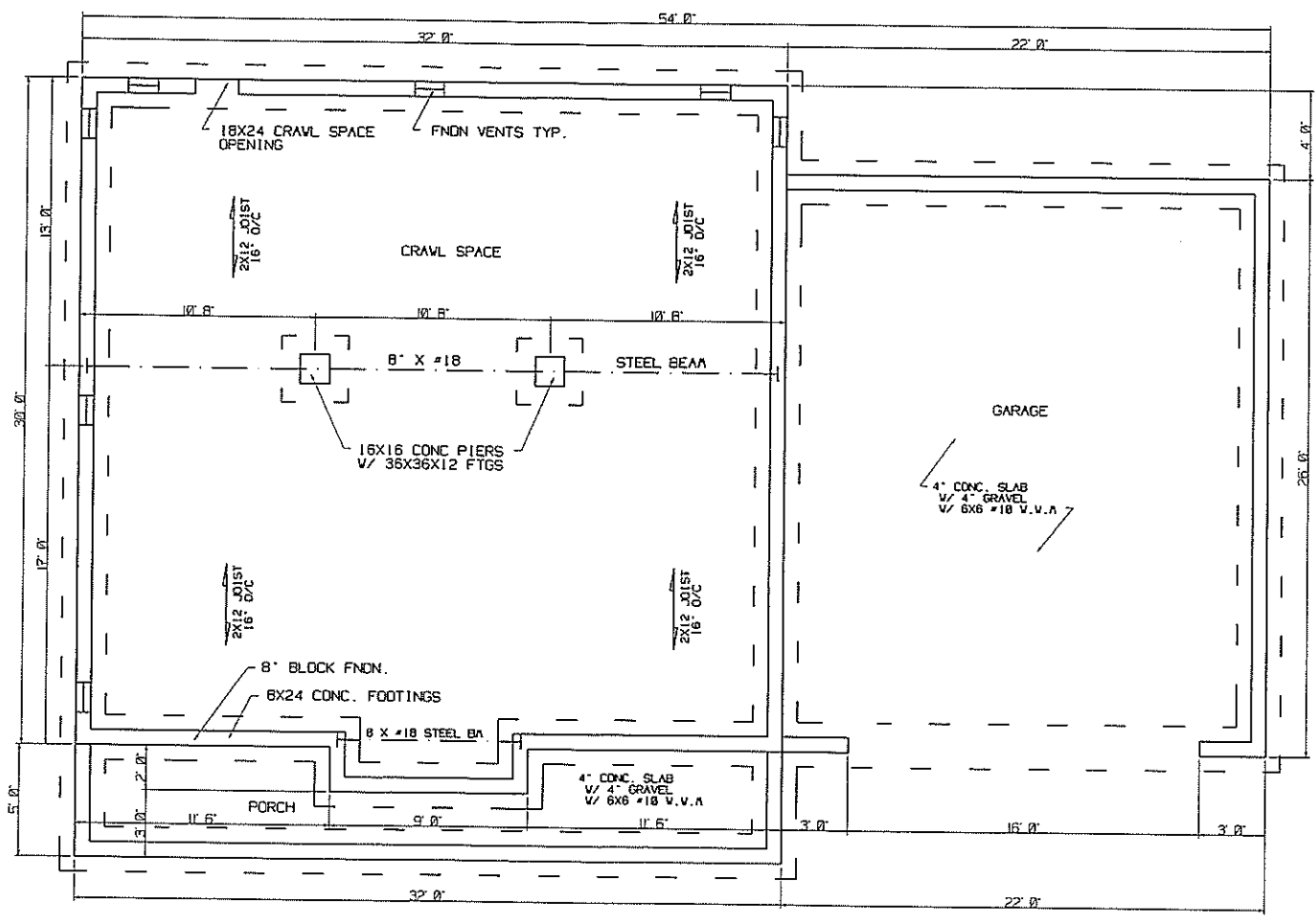
FOUNDATION PLAN SCALE: 3/16" = 1'
